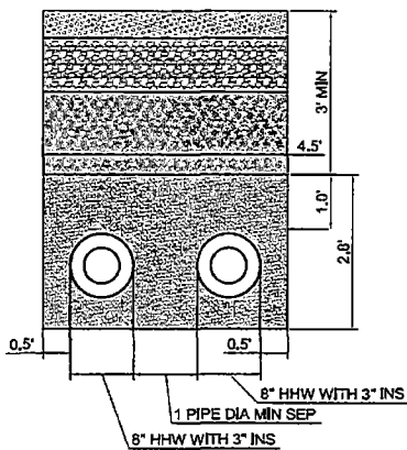
Figure 5: Heat Hot Water Trench - Maximum Section
