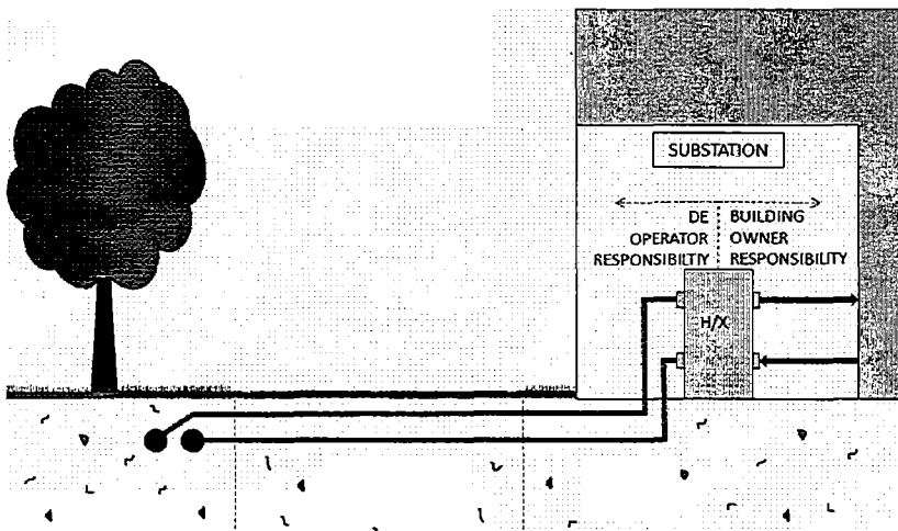
Figure 6: Substation Depiction
