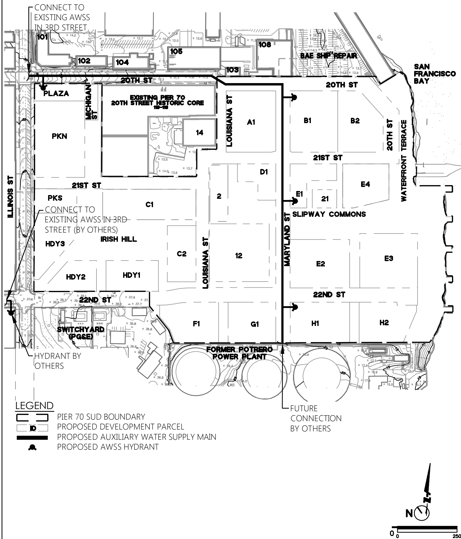
FIGURE 13.0: AUXILIARY WATER SUPPLY LOCATION
