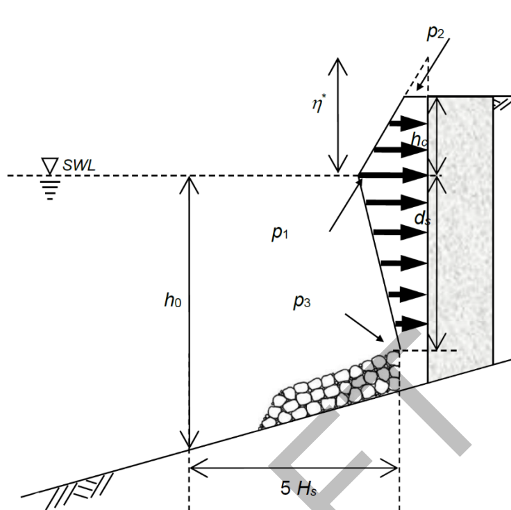
Figure 1612.6.5 (1) Nonbreaking wave horizontal loads on vertical walls
