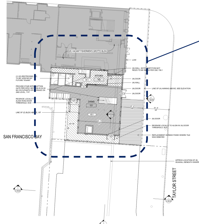
Site Plan
