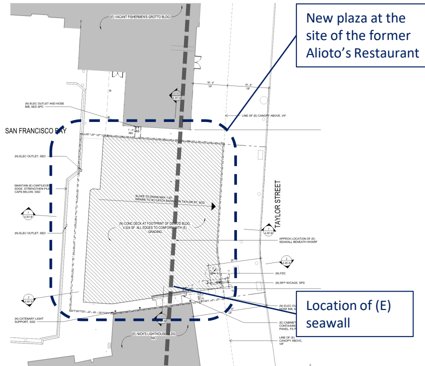
Site Plan
